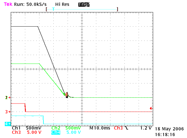
Figure 3. Disable Sequence
