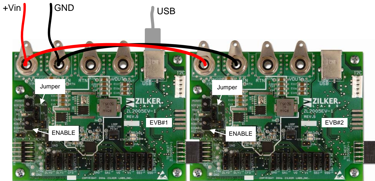
Figure 1. EVB Connections for Tracking
