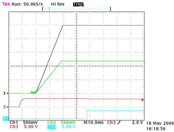
Figure 2. Enable Sequence
